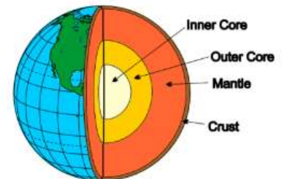
Layers of the Earth
